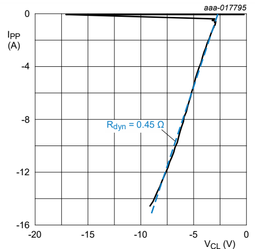
Fig. 8. Dynamic resistance with negative clamping voltage
