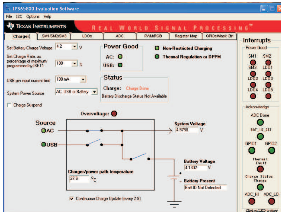
Figure 3. Charger Section
