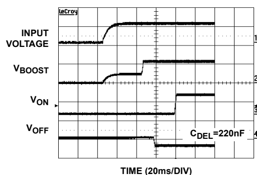
FIGURE 13. START-UP SEQUENCE
