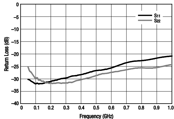
Figure 6. Return Loss Attenuation State
