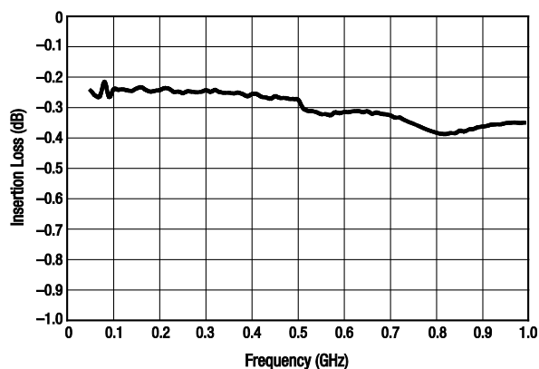
Figure 3. Typical Insertion Loss
