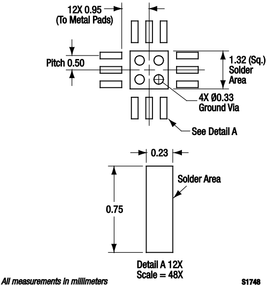
Figure 9. SKY12408-321LF PCB Layout Footprint
