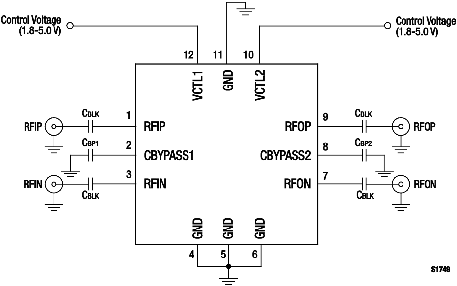
Figure 8. SKY12408-321LF Evaluation Board Schematic Diagram
