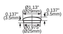
OB-31 Mounting Hole Rubber Plug
