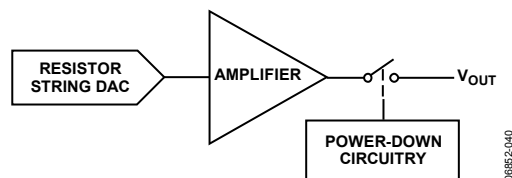
Figure 39. Output Stage During Power-Down
