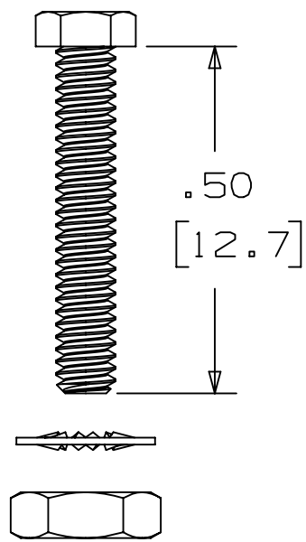
3341-6 HEX HEAD BOLT, NUT AND WASHER: BOLT - #2-56 X 1/2" MATERIAL: STAINLESS STEEL
