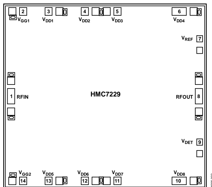
Figure 2. Pad Configuration
