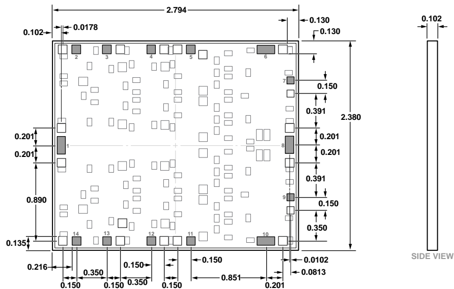
Figure 38. 14-Pad Bare Die [CHIP] (C-14-4)
