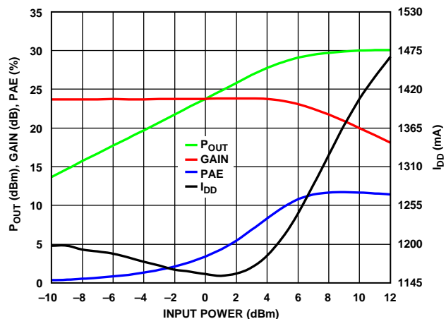
Figure 21. Power Compression at 39 GHz
