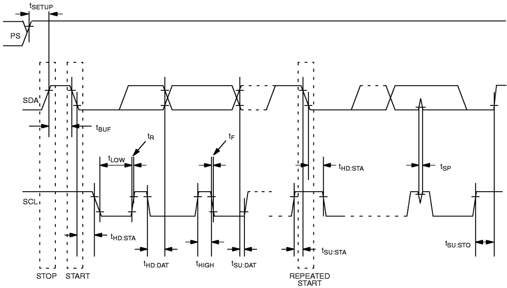
2-WIRE TIMING DIAGRAM Figure 8
