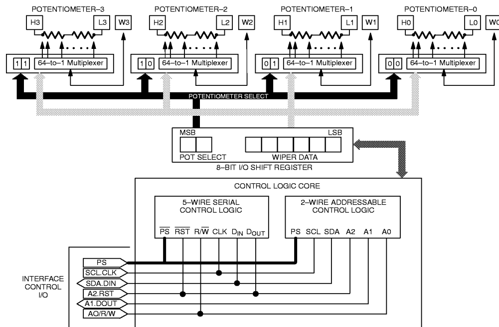
DS1844 BLOCK DIAGRAM Figure 1
