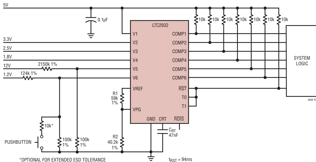
Figure 5. Six Supply Monitor with Hysteresis 5% Tolerance (Supplies Rising) 12.5% Tolerance (After \overline{\text{RST}} Goes High)
