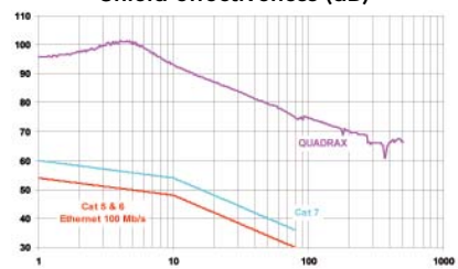
Shield effectiveness (dB)
