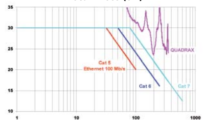
Return loss (dB)
