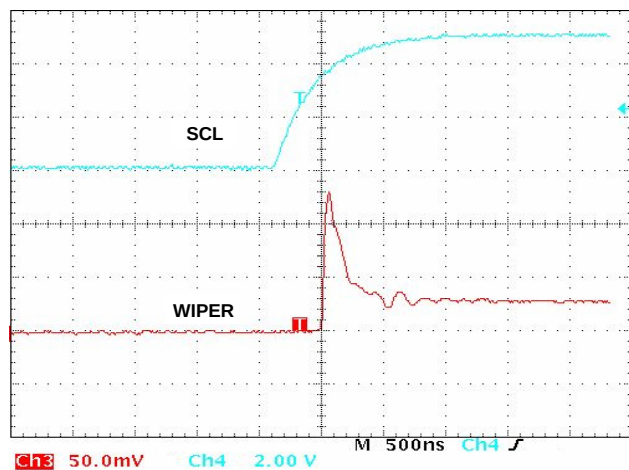
FIGURE 13. MIDSACLE GLITCH, CODE 7Fh TO 80h
