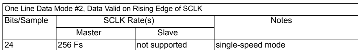
Figure 14. One Line Mode #2 Serial Audio Format
