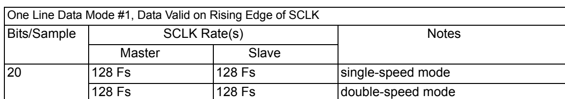
Figure 13. One Line Mode #1 Serial Audio Format
