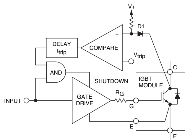
Figure 1. Desaturation Detector
