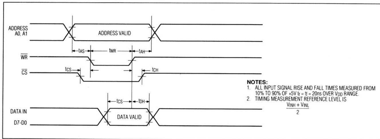
Figure 2. Write-Cycle Timing
