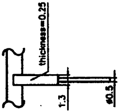
LEAD DETAILS
