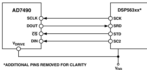
Figure 22. Interfacing to the DSP563xx
