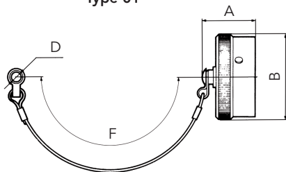
Cap for receptacle Type 01
