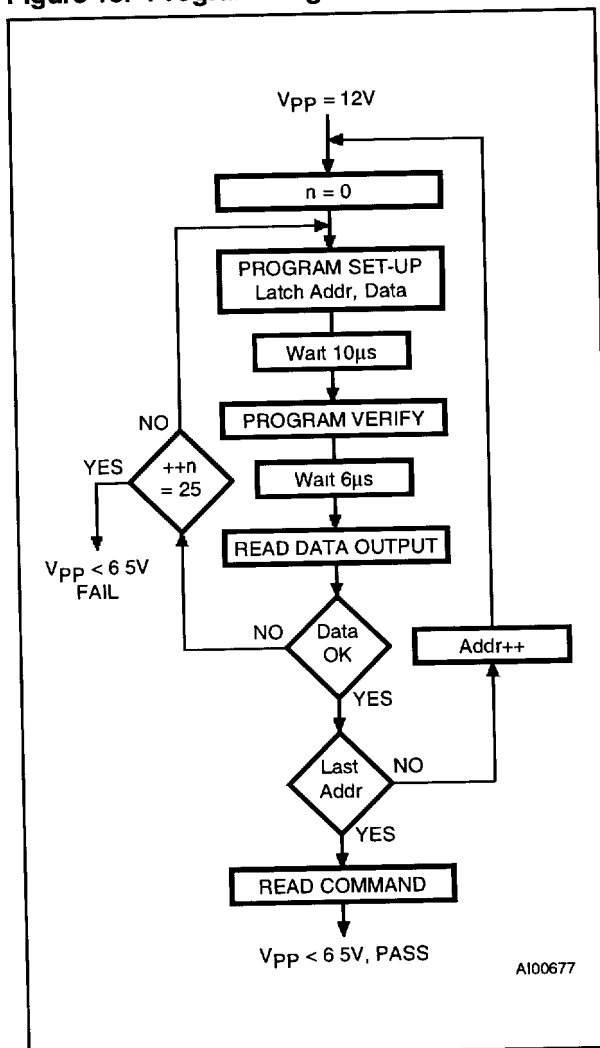
Figure 13. Programming Flowchart
