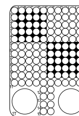
120T2 / 120Q2 118 #22 2 #8 Twinax/Coax/Quadrax (#8 Grounded to Shell)
