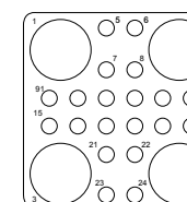
24T4 / 24Q4 20 #20 4 #8 Triax/Quadrax
