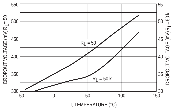
Figure 6. Dropout Voltage versus Temperature
