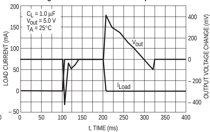
Figure 10. Load Transient Response
