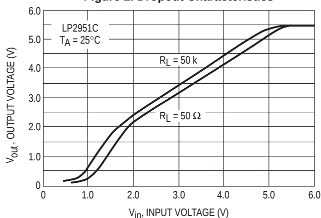
Figure 2. Dropout Characteristics
