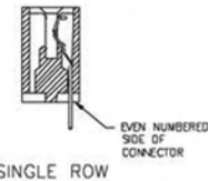
SECTIONS THROUGH CONTACT POSITION
