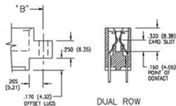
IN-CONTACT POLARIZING KEY
