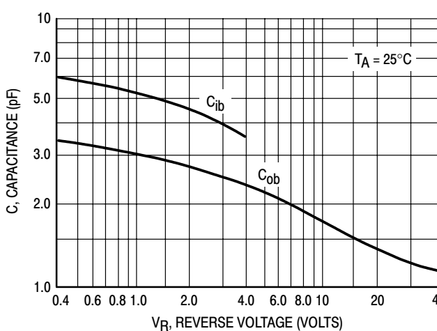
Figure 5. Capacitances
