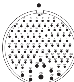
48-5 90 #16(A-BL,BN-BT,BW,BX) 1 #8(CD) 9 #12(BM,BU,BV,BY-CC,CE)
