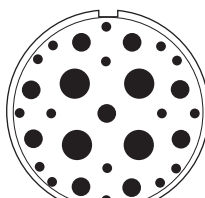
40-10 16 #16(A,B,E-H,M,N,P Q,V-Y,b,c) 9 #8(C,D,I,L,O,R,U,Z,a) 4 #4(K,J,S,T)
