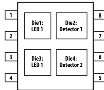
Figure 18. Diagram of ACPL-K74T/K75T for measurement
