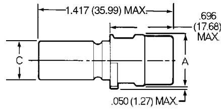
Plug
