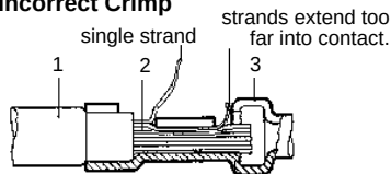
Incorrect Crimp
