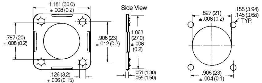
Mounting Dimensions
