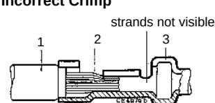
Incorrect Crimp
