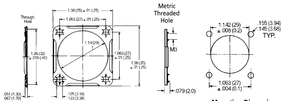
Mounting Dimensions
