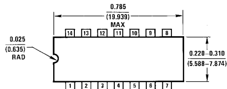
Ceramic Leadless Chip Carrier Package (E) Order Number 54LS03LMQB NS Package Number E20A
