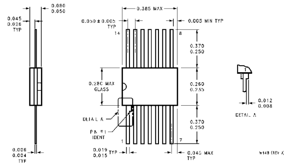
14-Lead Ceramic Flat Package (W) Order Number 54LS03FMQB or DM54LS03W NS Package Number W14B
