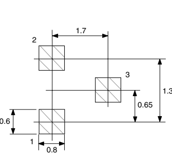
OUTLINE 30 RECOMMENDED P.C.B. LAYOUT
