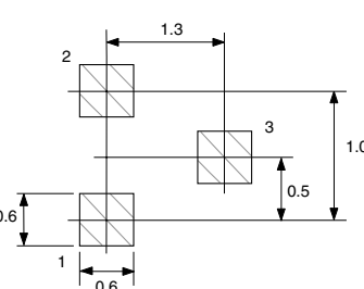
OUTLINE 19 RECOMMENDED P.C.B. LAYOUT
