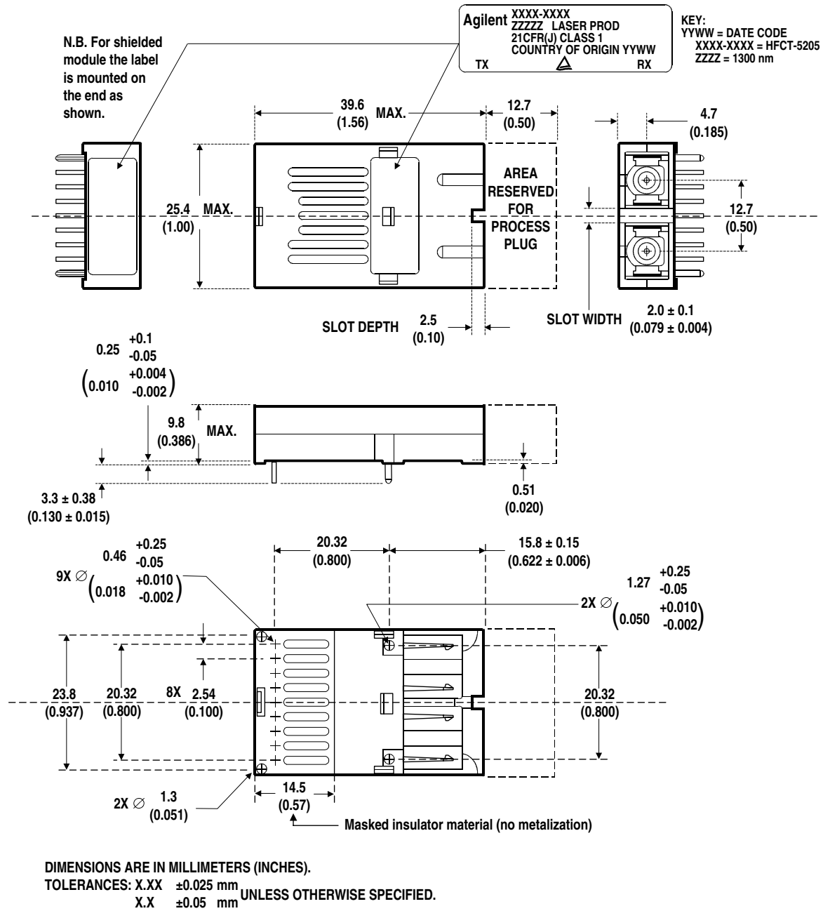
Figure 5. Package Outline Drawing for HFCT-5205
