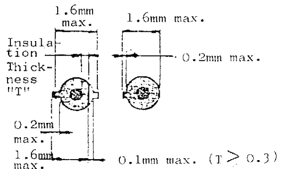
Detailed Cross-section Fig. 3-b
