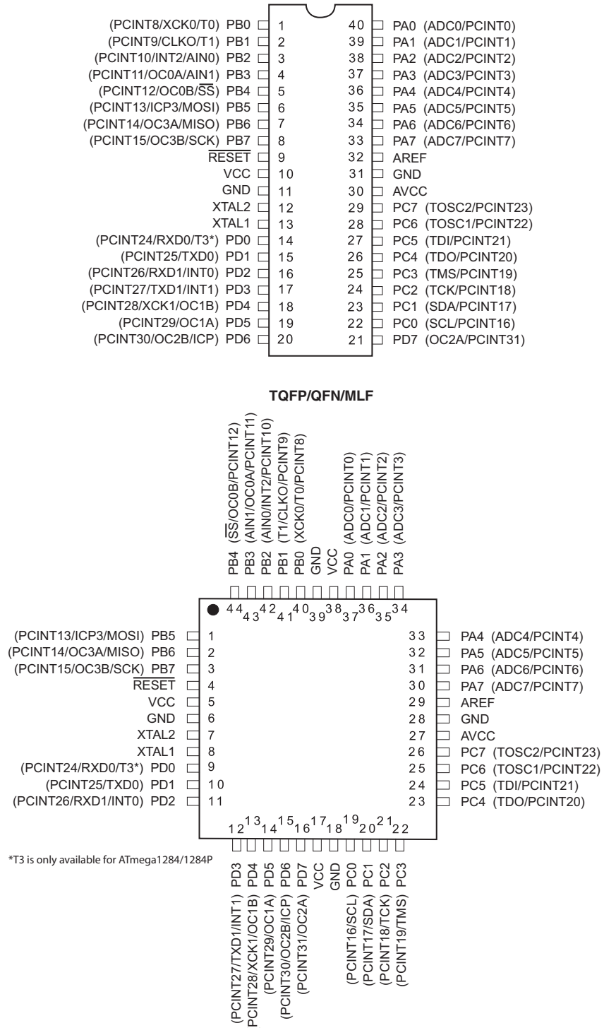
Figure 1-1. Pinout.
