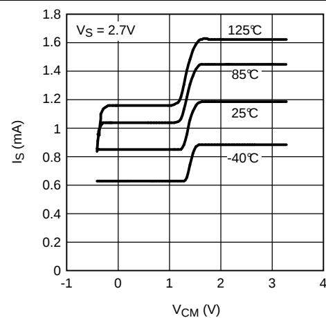
Figure 28. I_{\text{S}} vs. V_{\text{CM}} (LM7321)
