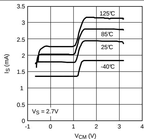
Figure 29. I_{\text{S}} vs. V_{\text{CM}} (LM7322)
