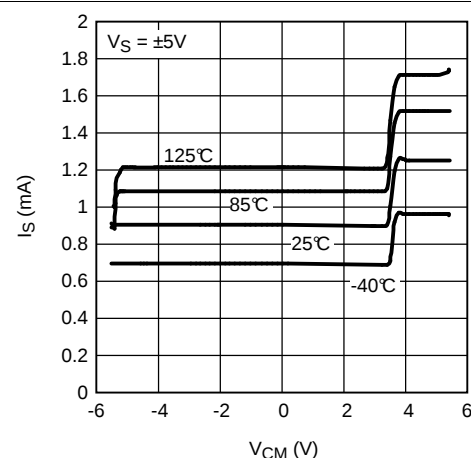
Figure 30. I_{\text{S}} vs. V_{\text{CM}} (LM7321)
