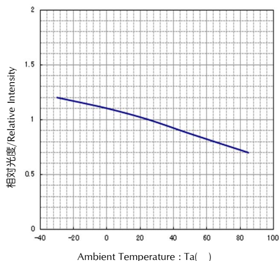
Ambient Temperature vs. Relative Intensity Condition : I_F = 10\text{mA}
