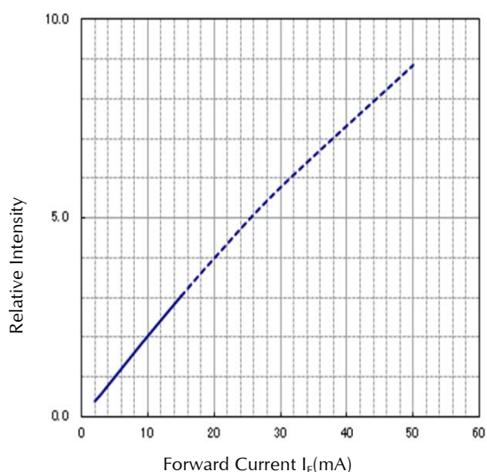
Forward Current vs. Relative Intensity Condition : T_a = 25
