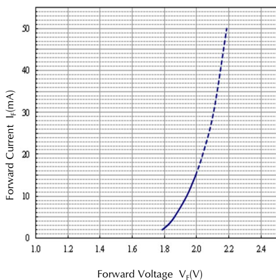
Forward Voltage vs. Forward Current Condition : T_a = 25
