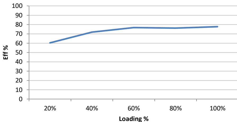
AM3T-0524S-RVZ Efficiency vs. Loading
