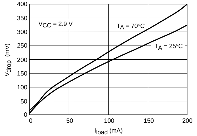
Figure 4. Dropout versus Load Current (Regulator R2)
