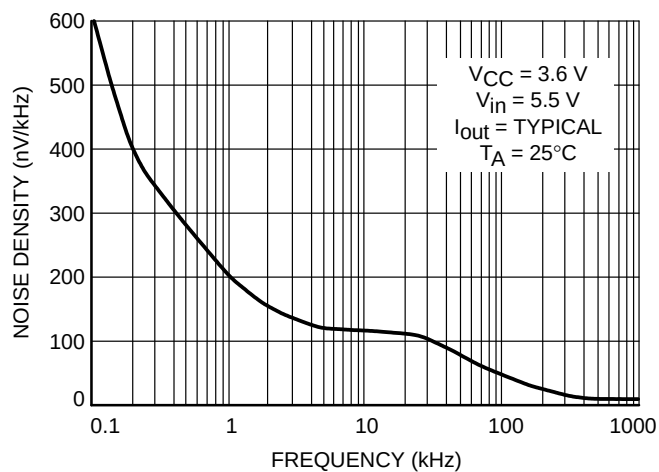
Figure 10. Output Noise Density versus Frequency (Regulators R6, R7)
