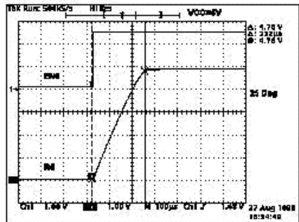
Figure 16. Enable response: Regulator 6
