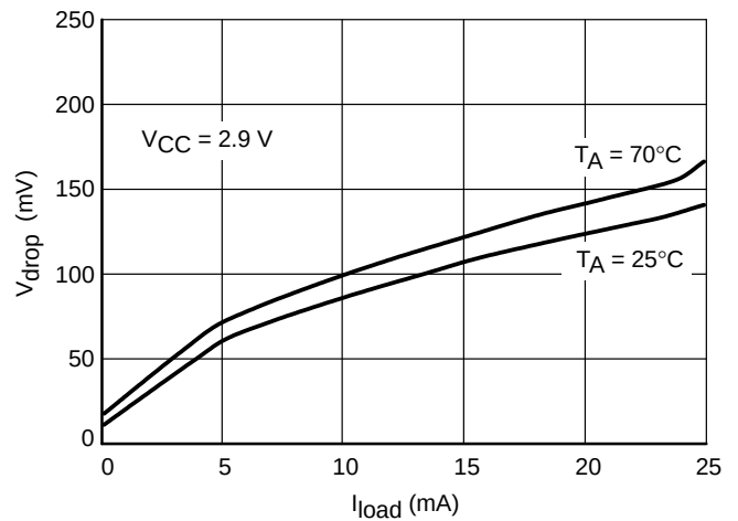
Figure 6. Dropout versus Load Current (Regulator R5b)
