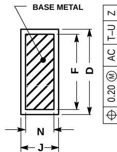
SECTION AE-AE
