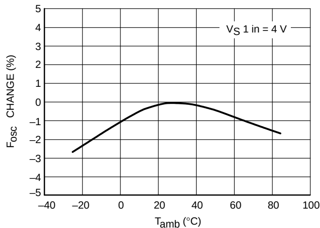
Figure 12. Normalized Charge Pump Oscillator Frequency Change versus Temperature
