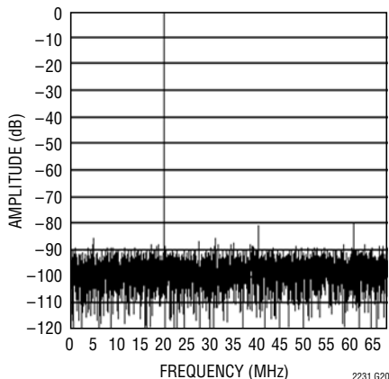
LTC2231: 8192 Point FFT, f_{IN} = 250\text{MHz} , -1dB, 2V Range
