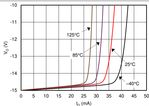
Figure 42. Output Swing to Rail While Sinking Current
