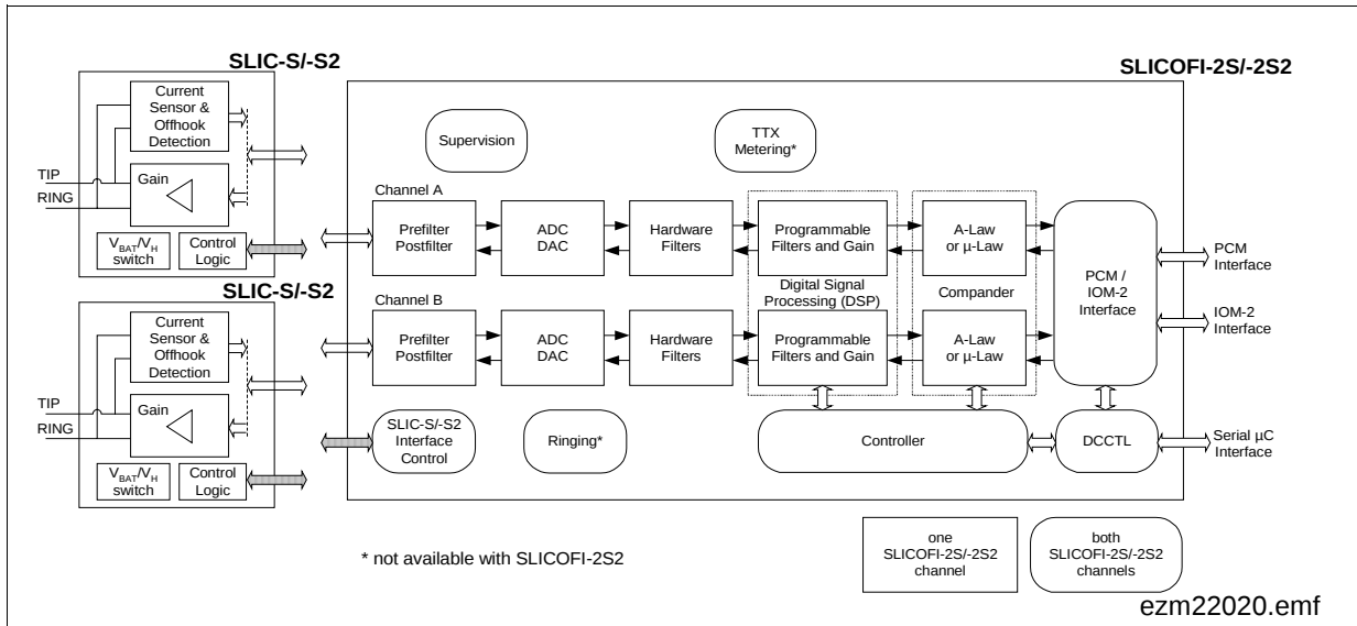
Figure 7 Line Circuit Functions included in the DuSLIC-SI-S2
