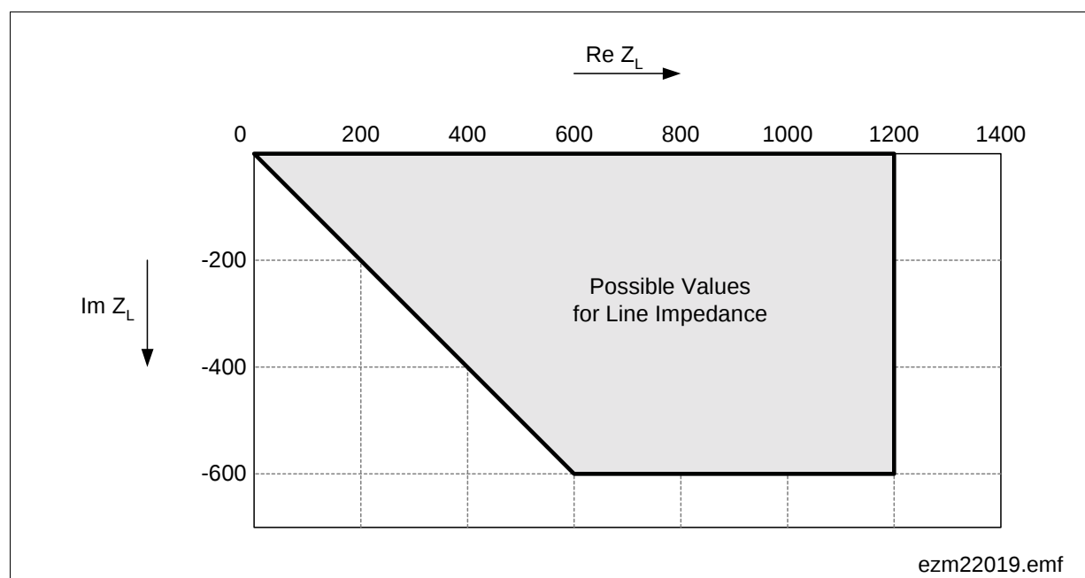
Figure 24 Nyquist Diagram
