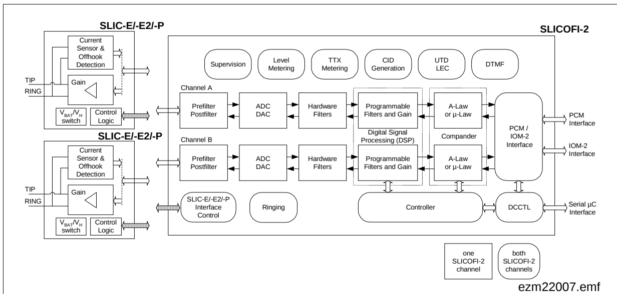
Figure 8 Line Circuit Functions included in the DuSLIC-EI-E2I-P
