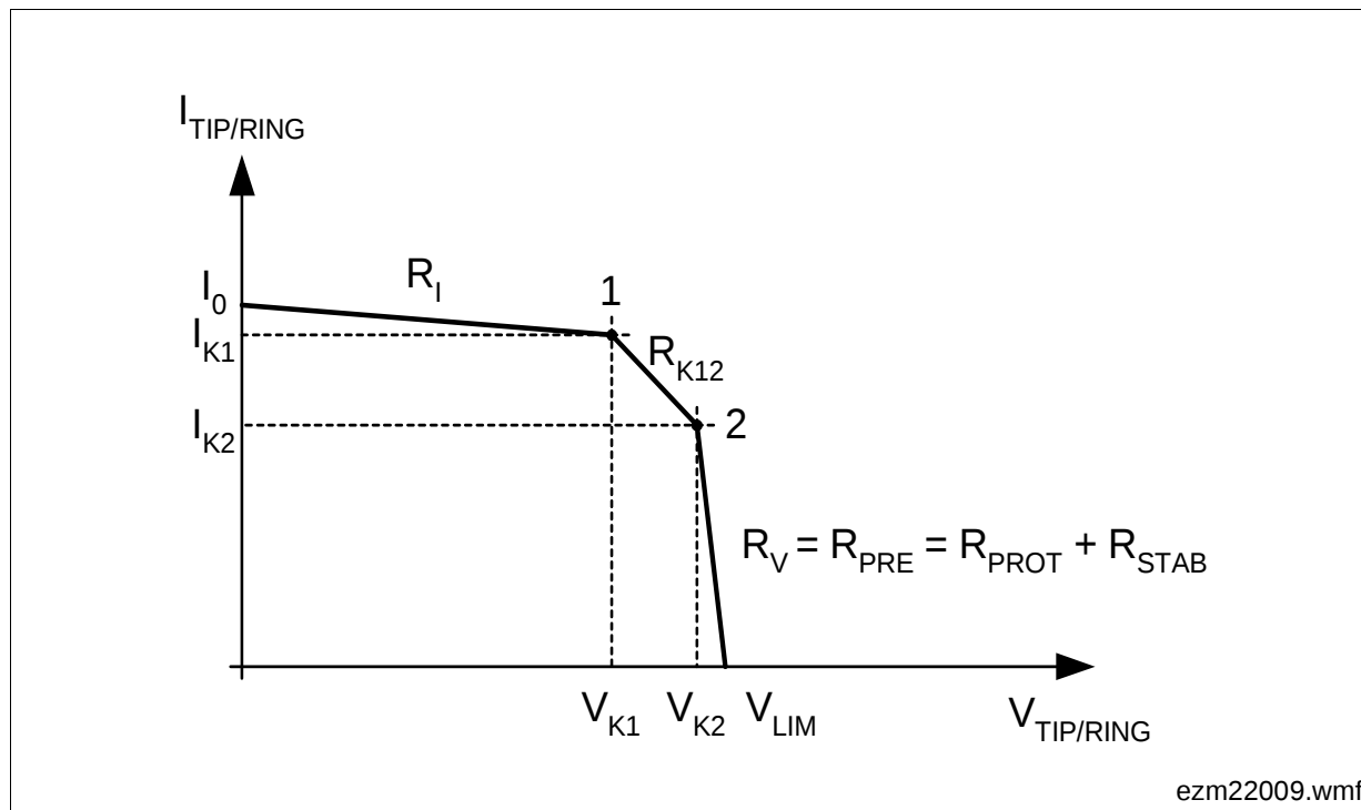
Figure 18 DC Characteristic
