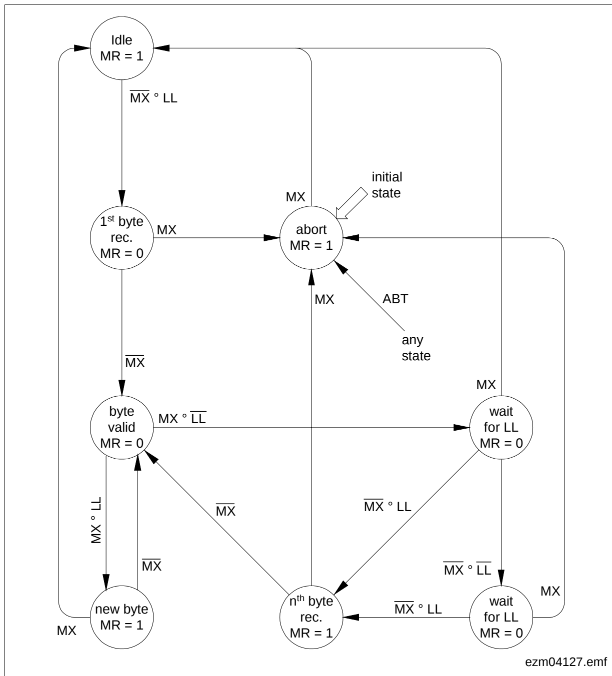
Figure 67 State Diagram of the SLICOFI-2x Monitor Receiver
