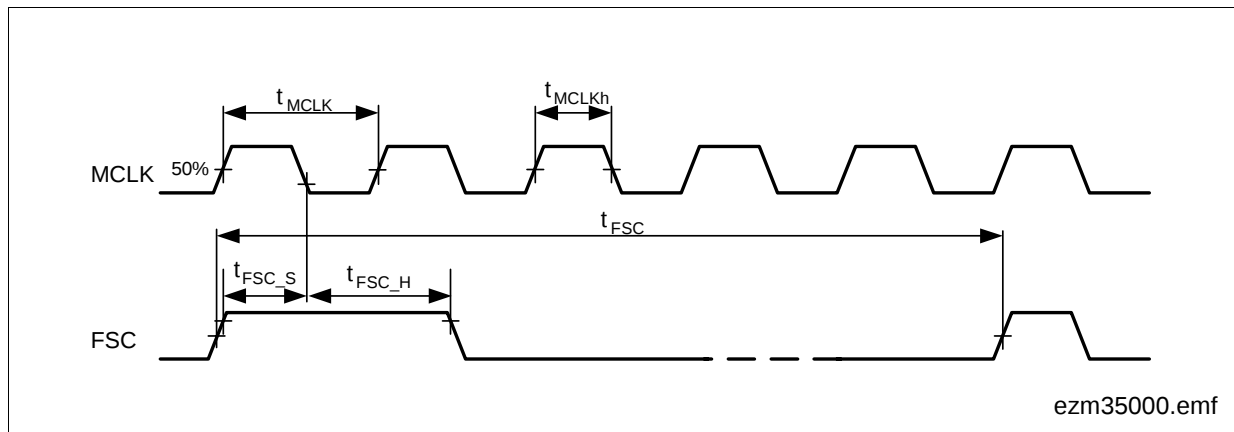
Figure 91 MCLK / FSC-Timing
