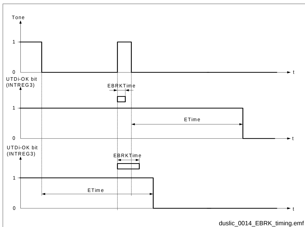
Figure 73 Example for UTD Tone End Detection Timing
