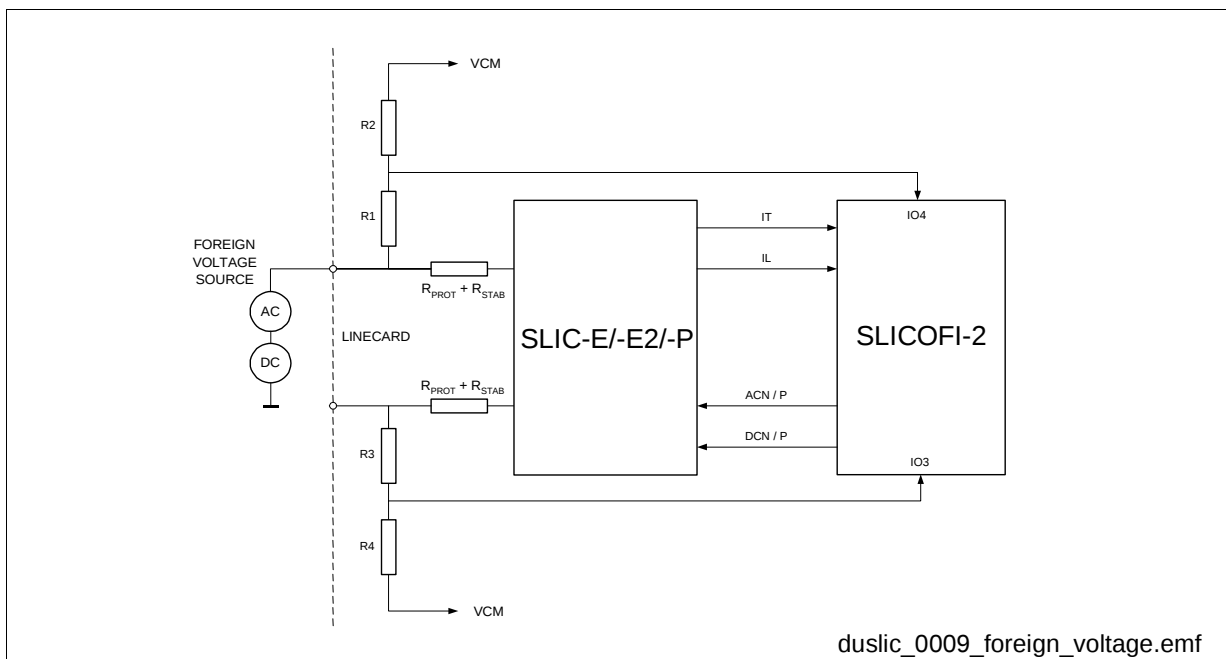
Figure 52 Foreign Voltage Measurement Principle
