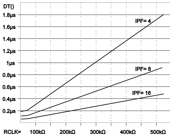
Fig. 3: Adjusting the minimum transition distance via resistor RCLK.
