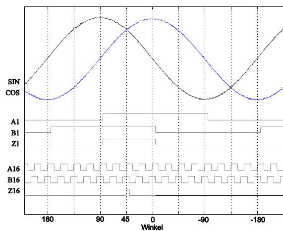
Fig. 12: ROT= hi, SIN leading COS
