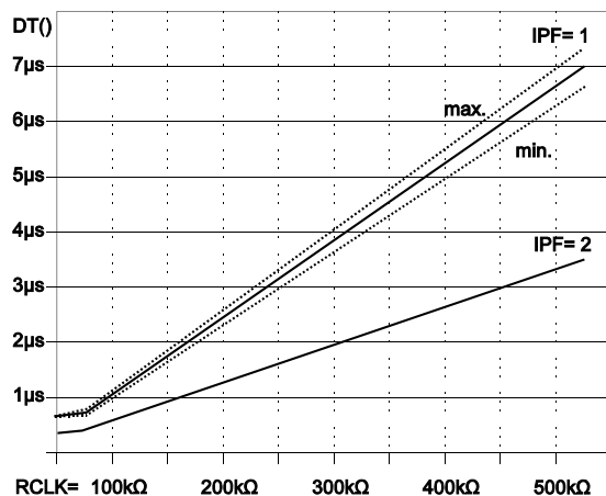
Fig. 1: Adjusting the minimum transition distance via resistor RCLK (given typical at 5V, 27°C; for IPF= 1 within 5V \pm 10% and -40..+125°C ranges).
