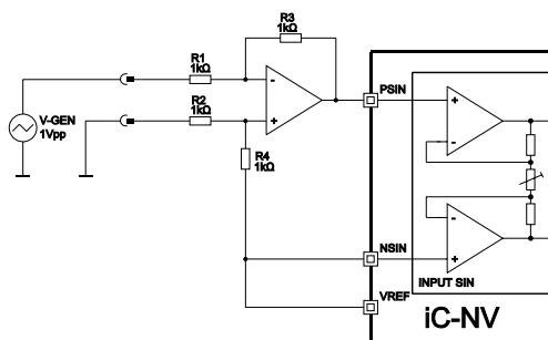
Fig. 16: Input circuit for single-side voltage or current source signals with ground reference (adaptation via resistors R3, R4).
