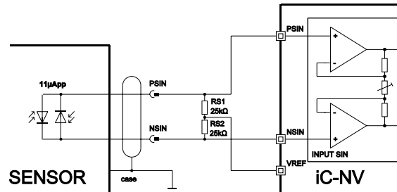
Fig. 15: Input circuit for current signals of 11μA. In this circuit offset adjustment is not possible.
