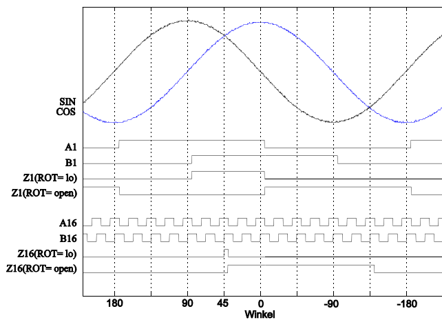
Fig. 10: ROT= lo/open, SIN leading COS
