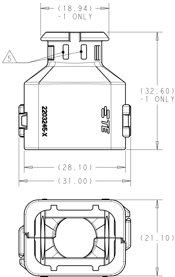
2292862-1 ASSEMBLED VIEW SHOWN
