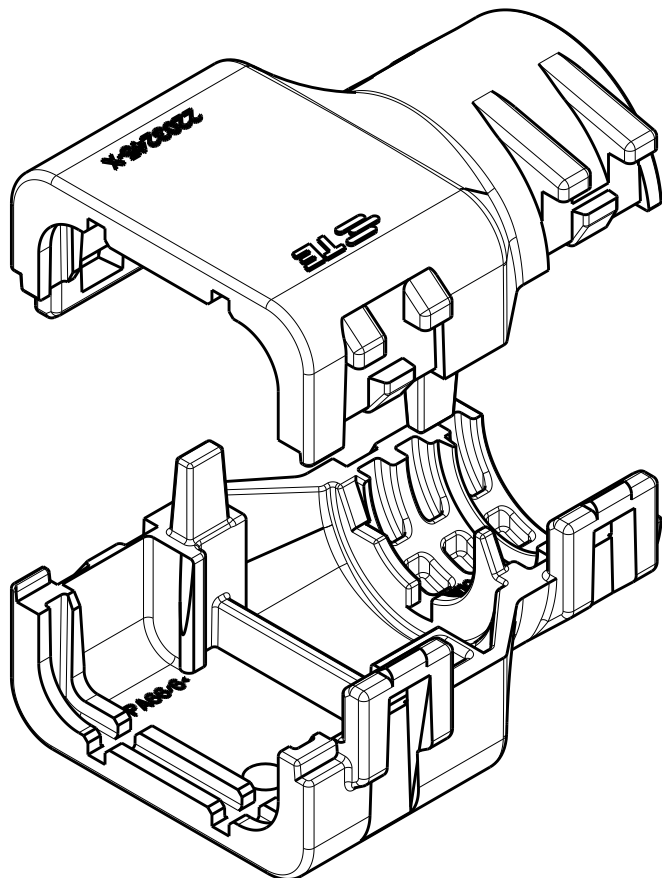
2292862-3 EXPLODED ISOMETRIC VIEW SHOWN
