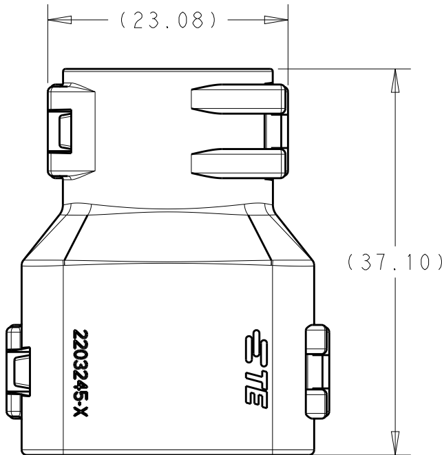
2292862-2 ASSEMBLED VIEW SHOWN
