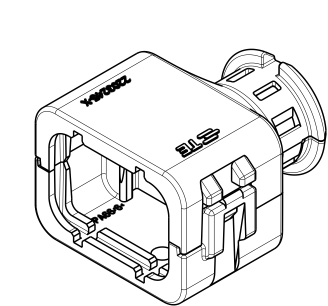
2292862-1 ASSEMBLED ISOMETRIC VIEW SHOWN
