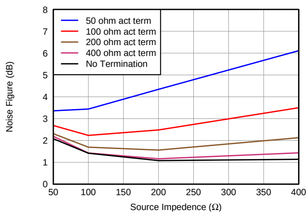
Figure 31. Noise Figure, LNA = 24 dB and Low Noise Mode
