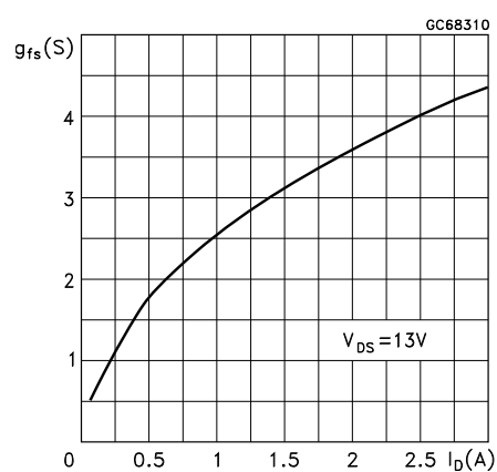
Figure 14. Transconductance
