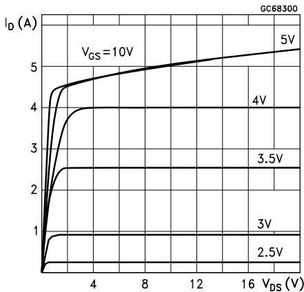
Figure 25. Output characteristics
