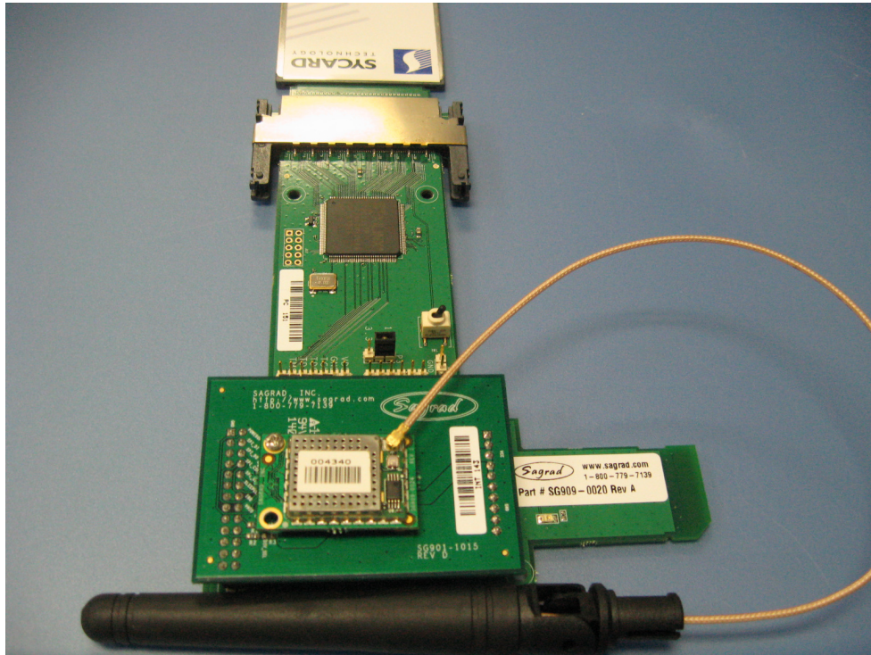
Boards assembled for PCMCIA application
