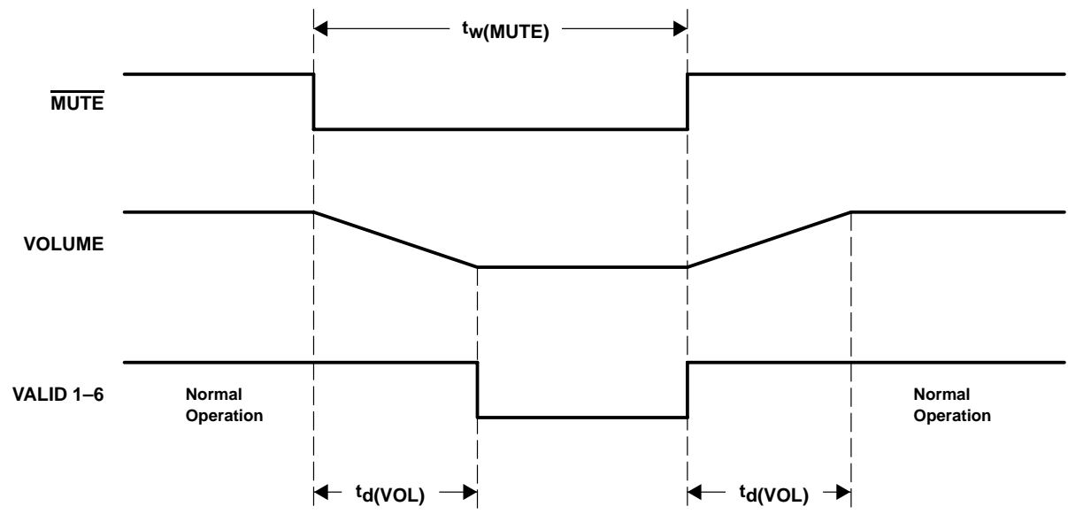
Figure 5–5. Mute Timing
