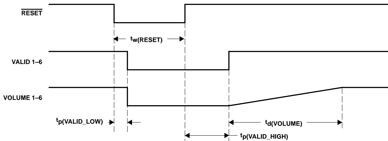
Figure 5–1. \overline{\text{RESET}} Timing
