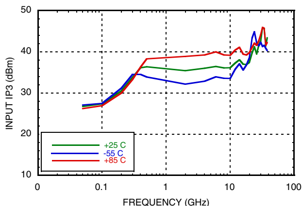
Input Third Order Intercept Point @-5V (Low Frequency Detail)
