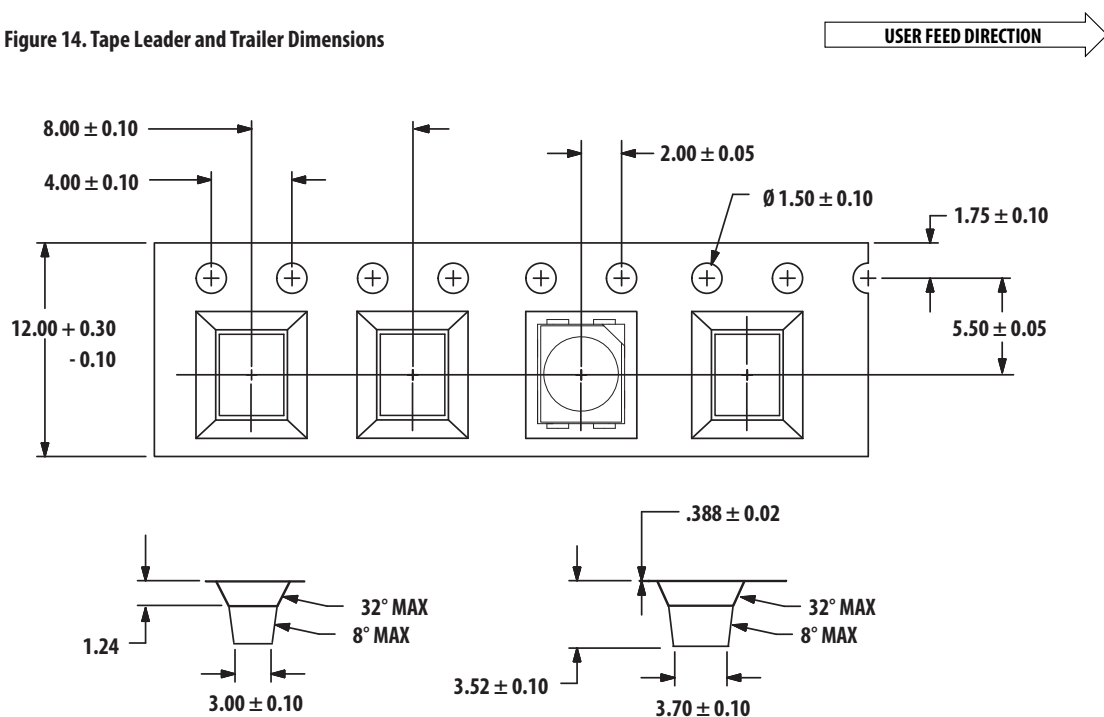
Figure 15. Tape Dimensions
