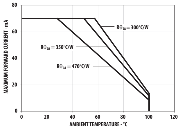
Figure 7a. Maximum Forward Current Vs. Ambient Temperature. Derated Based on T_{JMAX} = 110^\circ\text{C} , R_{\theta JA} = 300^\circ\text{C/W} , 350^\circ\text{C/W} and 470^\circ\text{C/W} (AllInGaP)
