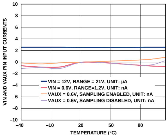
Figure 18. VIN/VAUX Input Currents vs. Temperature
