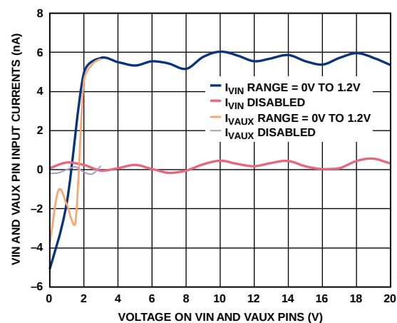
Figure 17. VIN/VAUX Input Currents vs. VIN/VAUX Voltage
