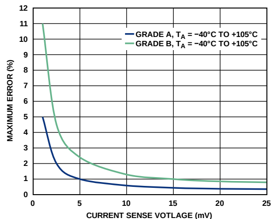
Figure 19. Worst Case Current Sense Error vs. Current Sense Voltage with 128 Sample Averaging, V_{\text{SENSEP}} = 0 \text{ V to } 18 \text{ V} , over Full Operating Temperature Range
