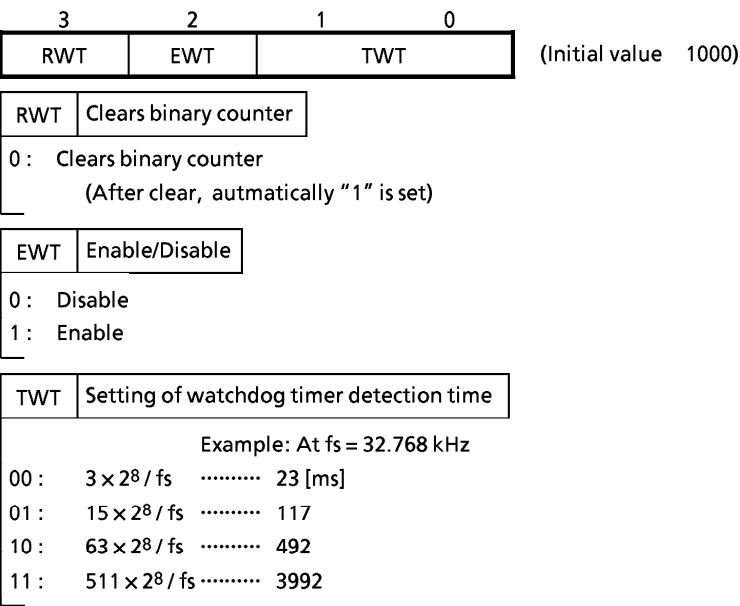
Figure 3-7. Command Register
