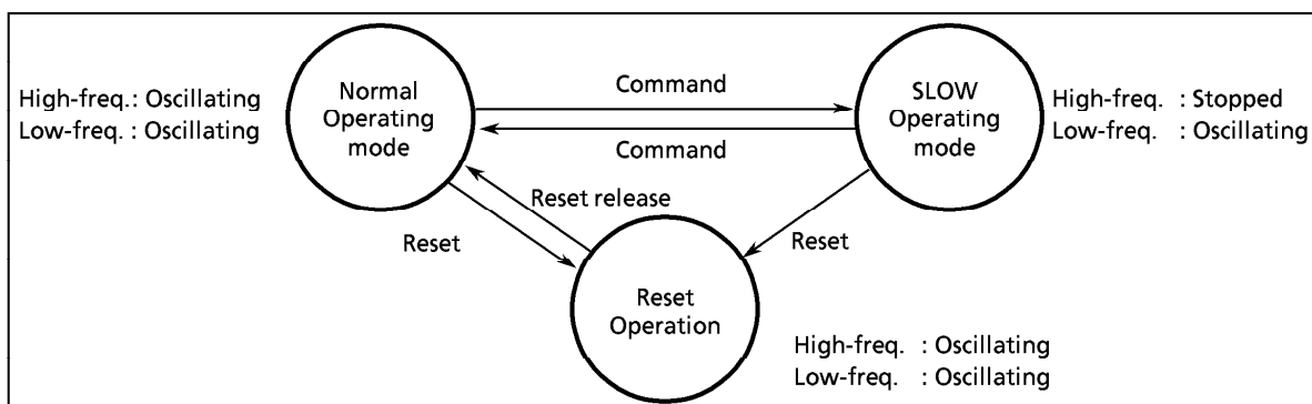
Figure 2-2. Operating Mode Transmission Diagram
