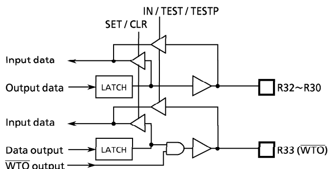
Figure 3-2. Port R3
