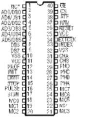
Fig. 1 *Should be left floating.
