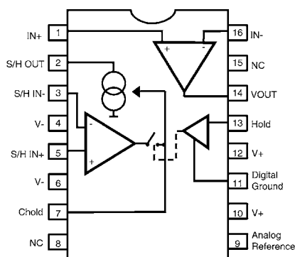
EL4093 (16-PIN PDIP, SO) TOP VIEW
